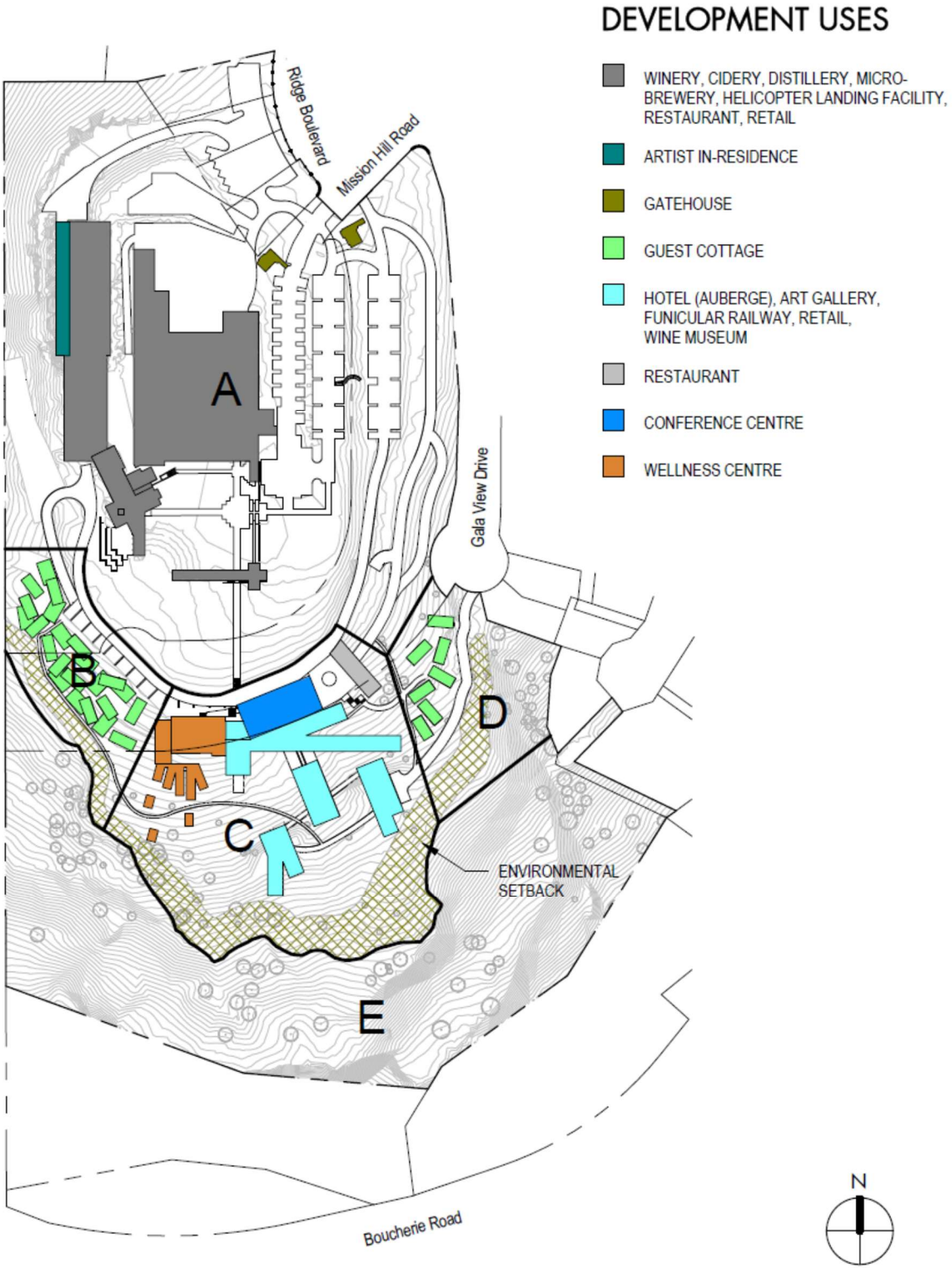
FIGURE 3 - SITE PLAN
